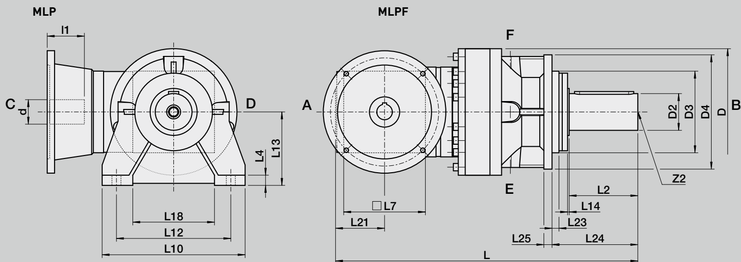
Motor dimensions
