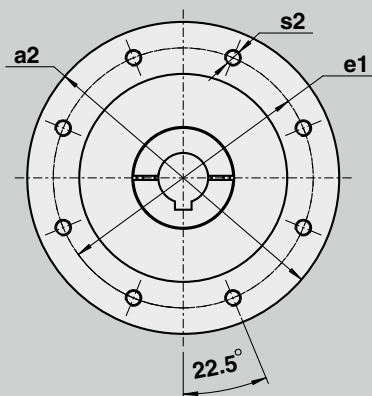
8x threaded mounting bores
